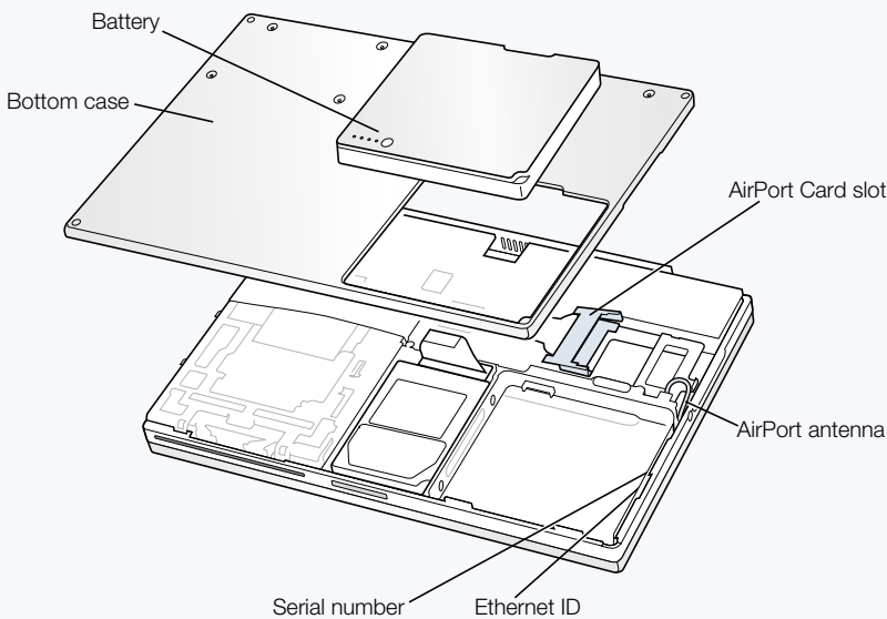
PowerBook turned over with the bottom case removed
