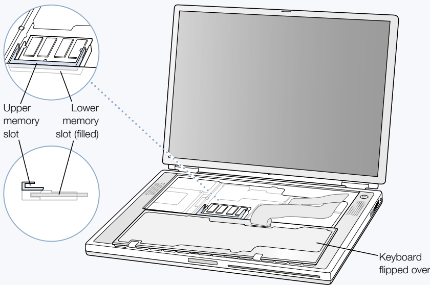
PowerBook with the keyboard flipped over and internal RAM slot visible
